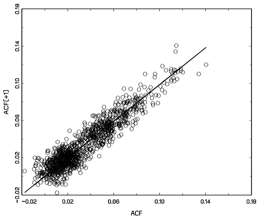
Figure 2: Scatterplot of empirical autocorrelations of z_t = \log y_t^2 , \gamma(k+1) (vertical axis) vs \gamma(k) (horizontal axis), k = 1, \dots, 1000 . The straight line is the no intercept regression line with slope 0.986 obtained using the first 100 observations of (\gamma(k), \gamma(k+1)) .
