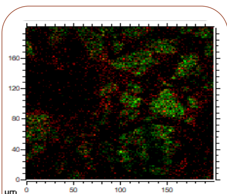
ToF-SIMS
