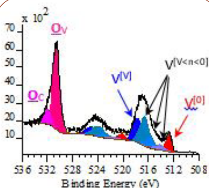
XPS
